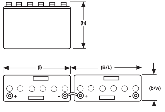
12 V block
