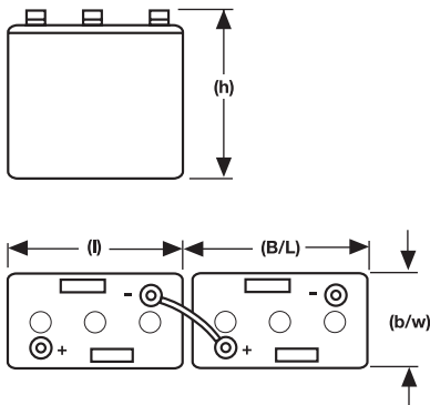
6 V block
